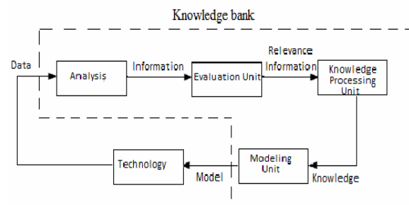
Fig. 1 KM model
